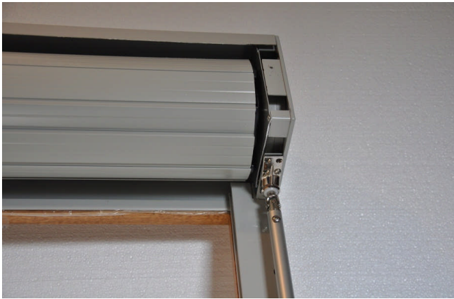
7. Temporarily attach crank to install slat
